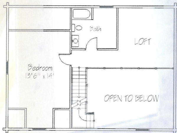
Second Floor 546 Square Feet
